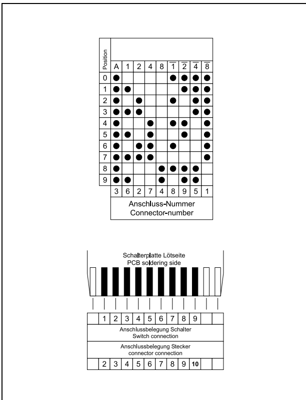
Code 044 BCD positive + complement - make before break contacts
